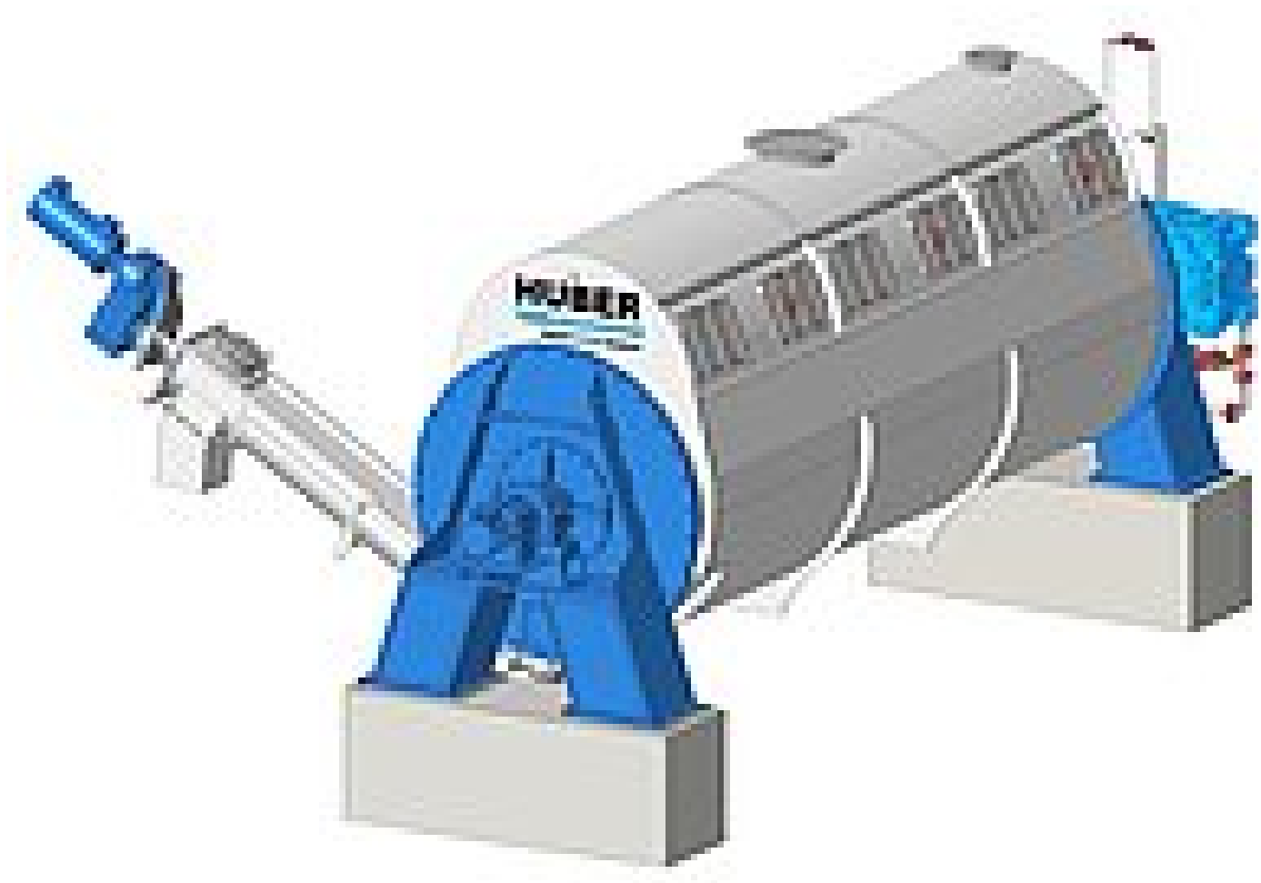
Figure 2: Schematic diagram of a HUBER Disc Dryer RotaDry® 2050
